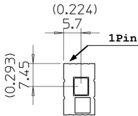
図 17 吸着位置 (from board edge)
